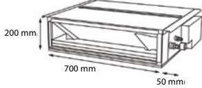
Baureihe A (15, 20, 25, 32)
